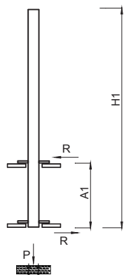
內爬框外廓尺寸 Overall dimensions of the internal climbing frame
