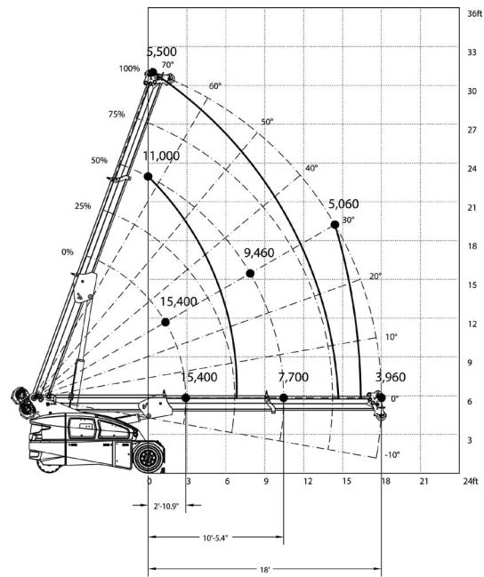
Short Wheelbase - Crossbar Deployed Winch
