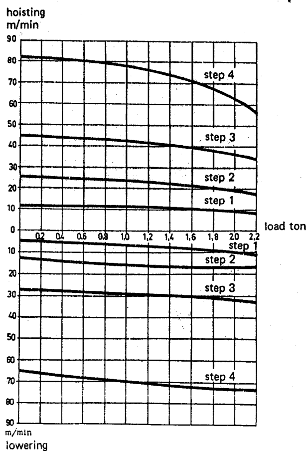
HOISTING/LOWERING SPEEDS in 4 steps
