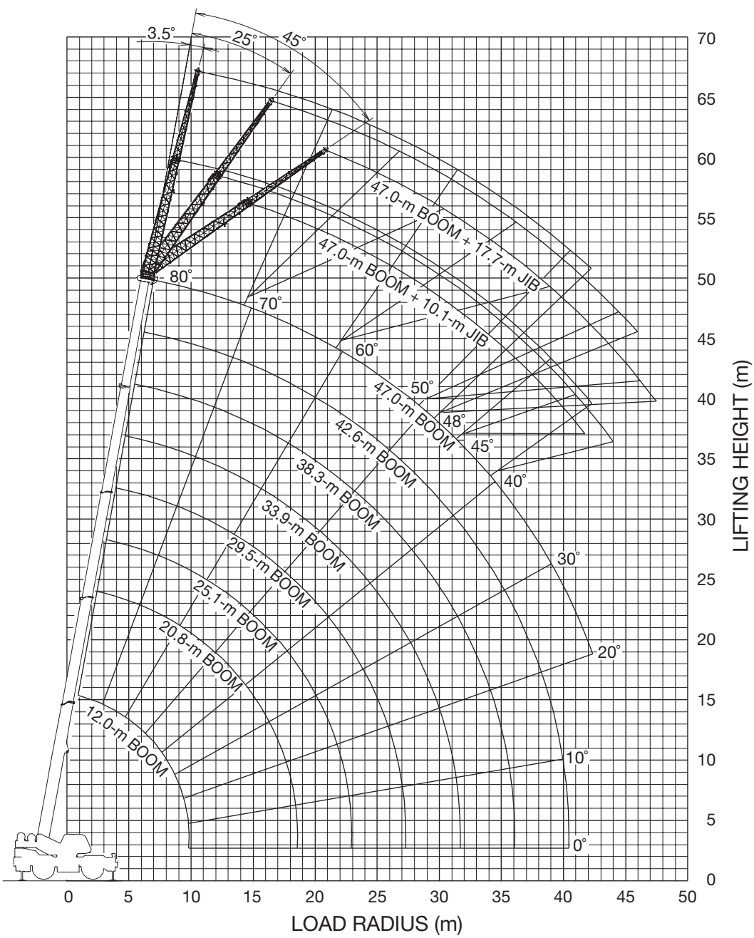
JIB
