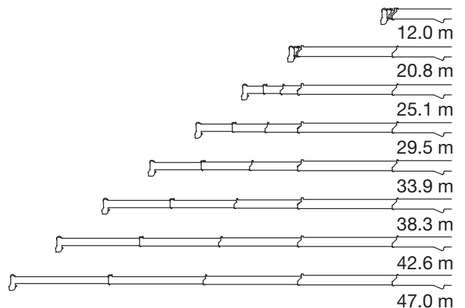
Boom Length
