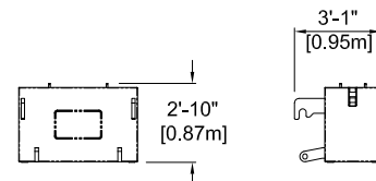
Carbody Counterweight 2 Pieces Weight: 10,000 lbs (4535kg)
