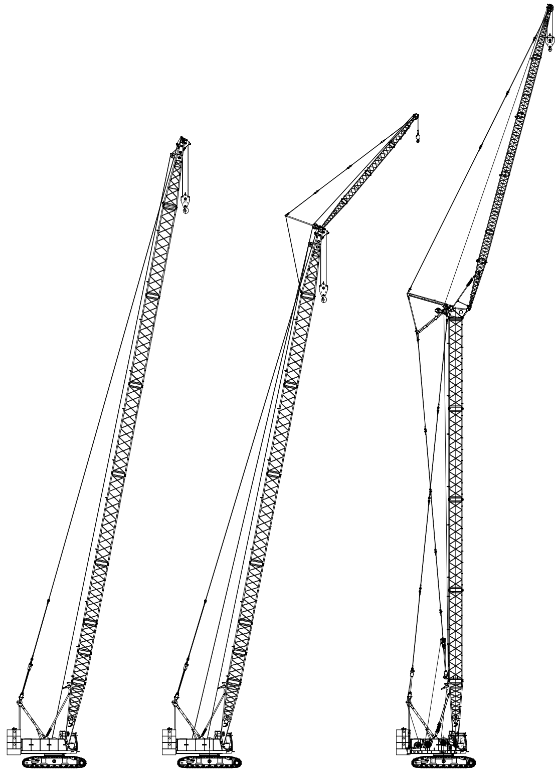
H Operating Condition: 13m-61m FJ Operating Condition: Boom 37-52m, Jib 9m-18m LJ Operating Condition: Boom 25.3m-43.3m, Jib: 19m-31m
