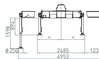
Sockel breit Crane base wide
