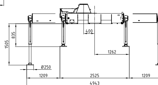
Socket Crane base
