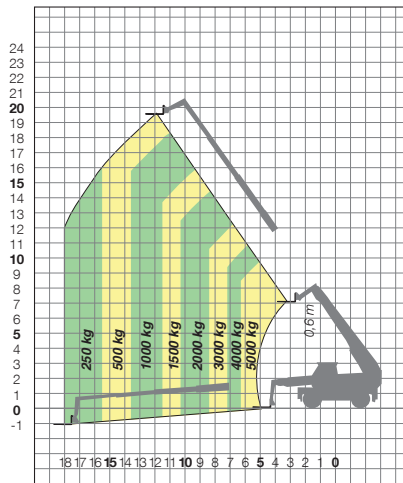
ROTO 60.24 MCSS FORKS ON FRONT TYRES
