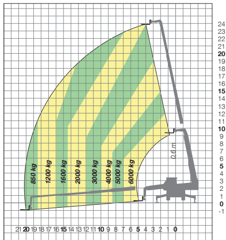
ROTO 60.24 MCSS FORKS ON STABILISERS ON 360°
