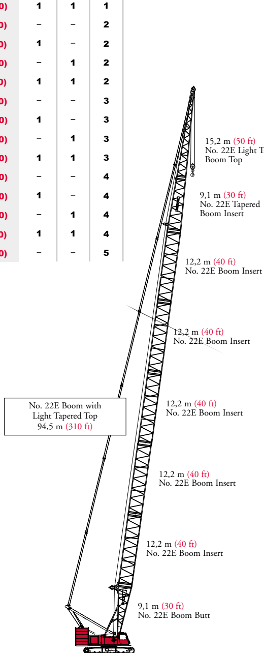
Model 999 Series 3 No. 22E Boom with Light Tapered Top 94,4 m (310 ft)
