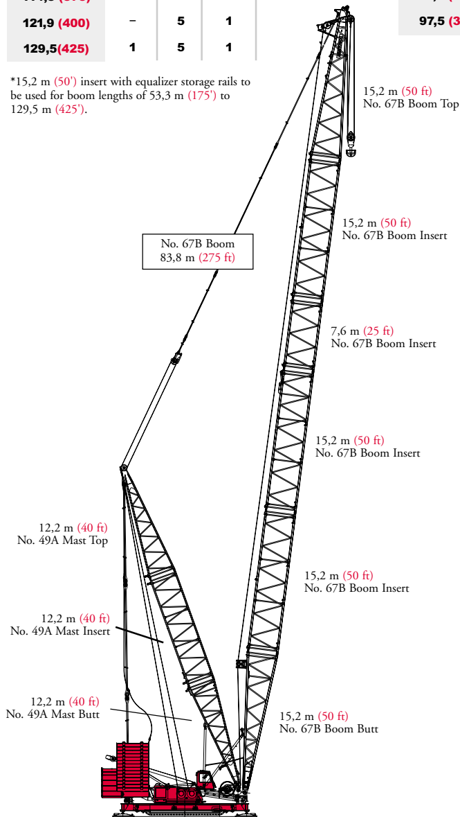
Model 999 RINGER® No. 67B Boom with No. 49A Mast Maximum Boom: 129,6 m (425 ft)
