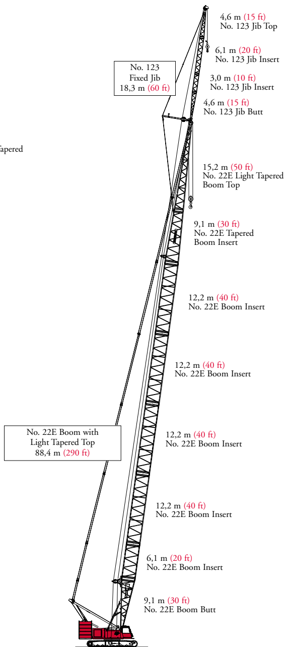
Model 999 Series 3 No. 123 Fixed Jib on No. 22E Boom with Light Tapered Top 106,7 m (350 ft)
