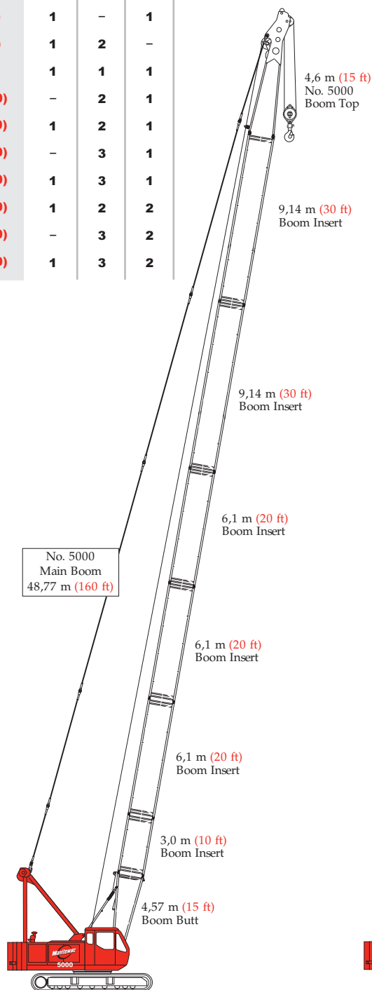
Model 5000 Main Boom 48,77 m (160 ft)
