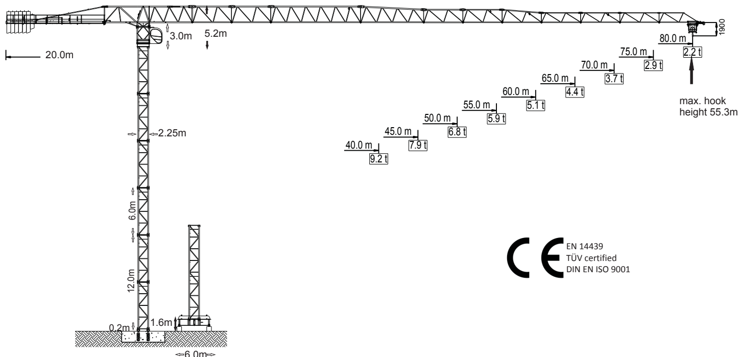
jib length & max. load with single / double trolley
