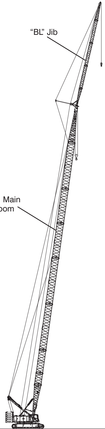
60–270 ft (18.29–82.30m) Main Boom With 30–90 ft (9.14–27.43m) Jib
