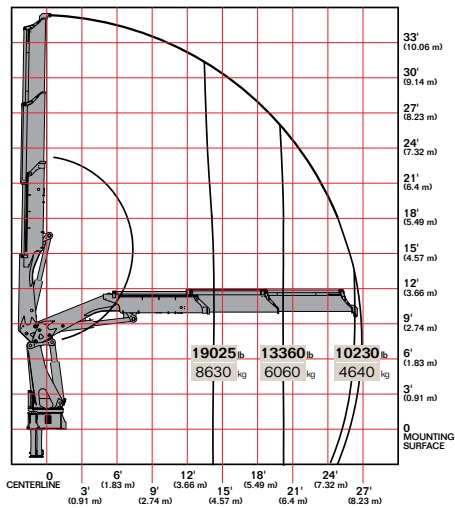
40/275 K2
