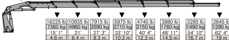
40/275 - 8 Hydraulic
