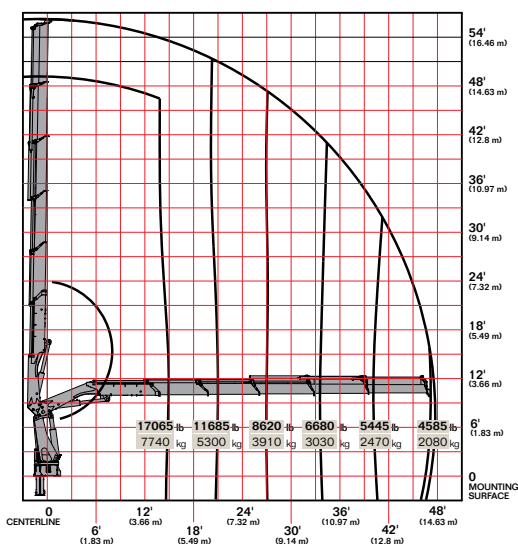
40/275 K5
