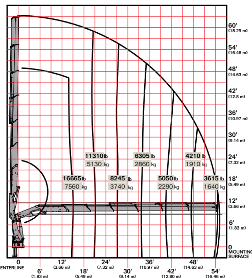
40/275 K6
