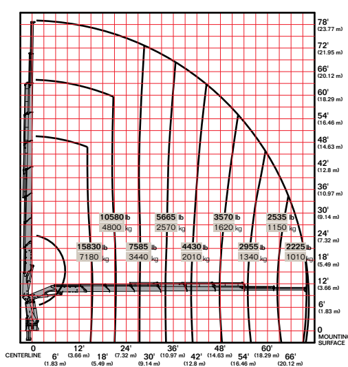
40/275 K8
