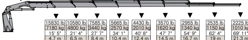
40/275 - 8 Hydraulic
