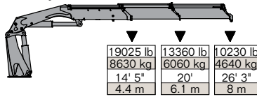
40/275 - 3 Hydraulic
