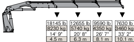
40/275 - 4 Hydraulic
