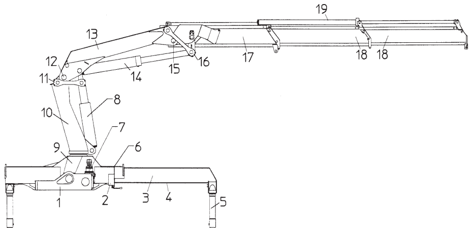
COMPONENT REFERENCE
