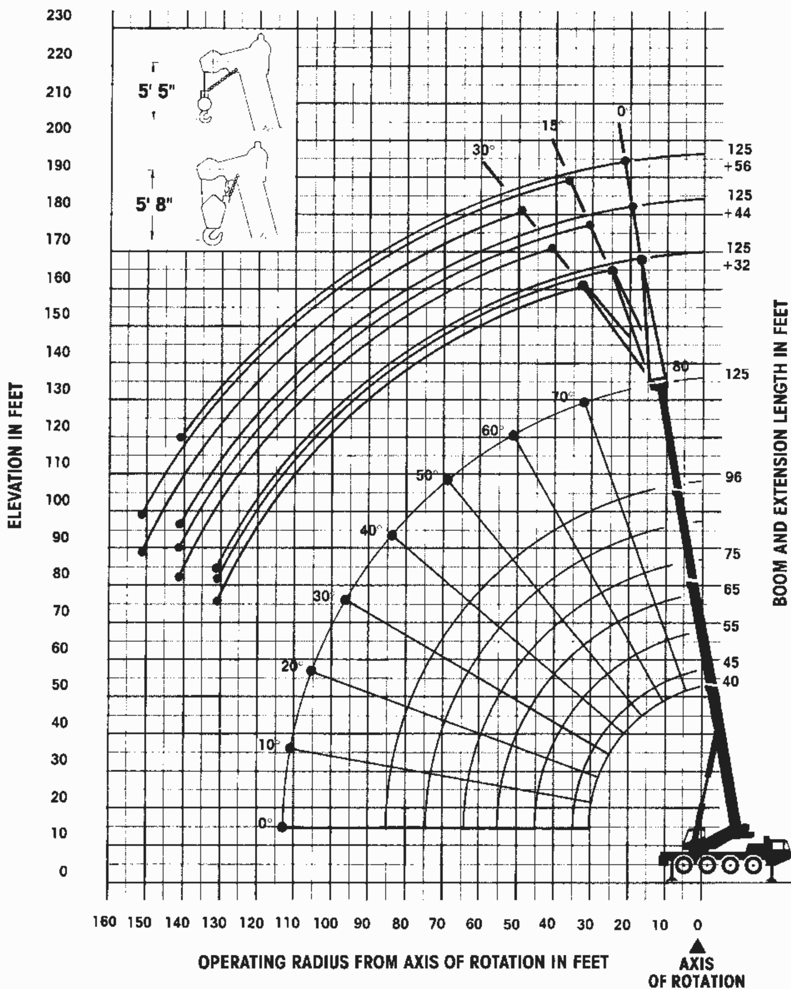
RANGE DIAGRAM (UNLADEN BOOM)
