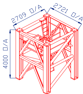
TOWER TYPE 442
