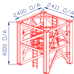
TOWER TYPE 392
