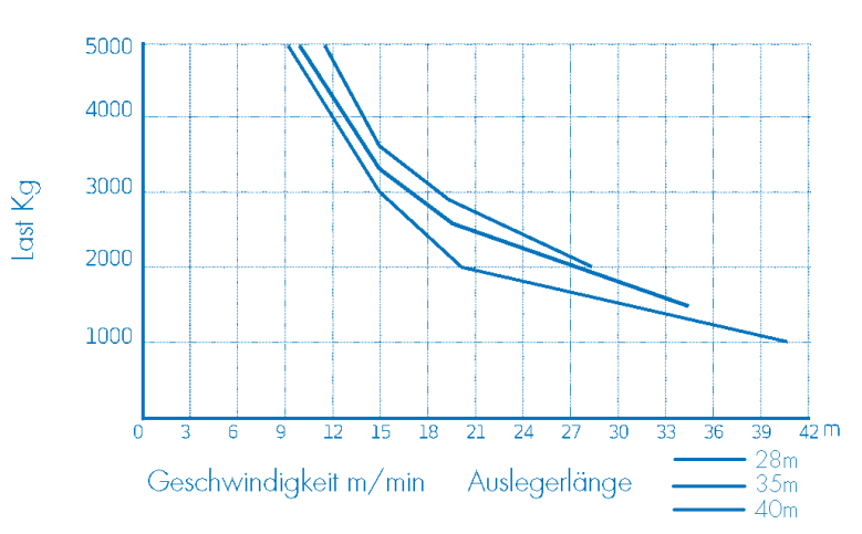
Last-Diagramm
