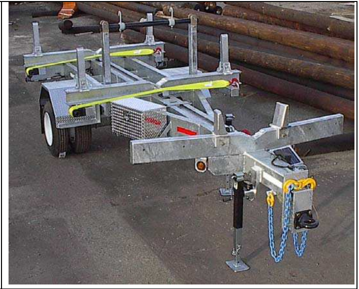
Unit equipped w/ Sliding Stanchions & Pole Chocks
