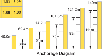
Outrigger Stationary
