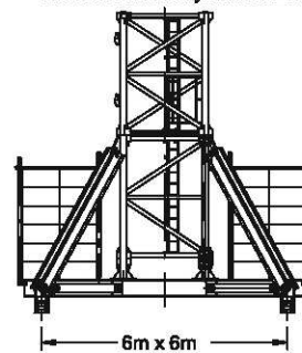
Chassis Stationary/Rail Mounted
